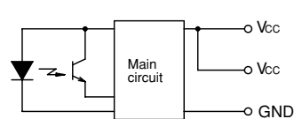
J Photo IC output (Open collector, Light on—Output transistor off)
