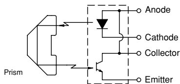
U Regressive Reflection Type Photosensor (anode and collector in common)
