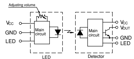
X Separate Type Photosensor (Sync light modulation system)
