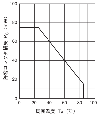
Collector Power Dissipation vs. Ambient Temperature
