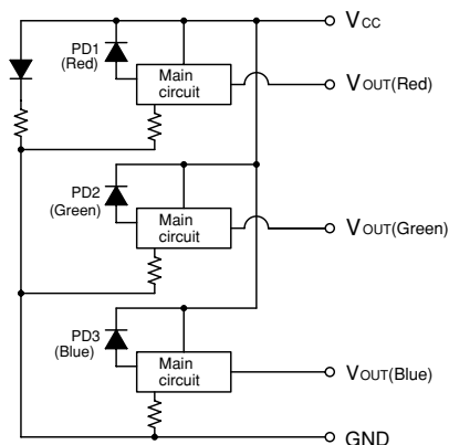
Y 3-Channel (R/G/B) independent analog output
