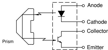
S Regressive Reflection Type Photosensor
