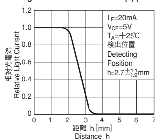
Detecting Position Characteristics (1) (Reference)
