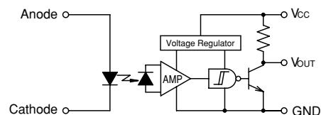
F Photo IC output (With pull-up resistor, Light on—Output transistor on)
