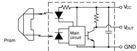
V Regressive Reflection Type Photosensor (Sync light modulation system)
