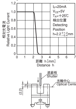
検出位置特性 (1) (参考) Detecting Position Characteristics (1) (Reference)
