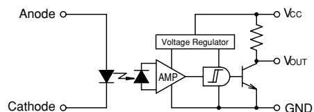
E Photo IC output (With pull-up resistor, Light on—Output transistor off)
