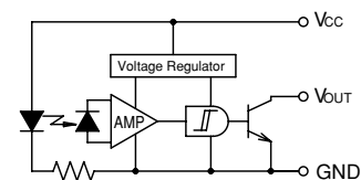
L Photo IC output (With pull-up resistor, Light on—Output transistor on)
