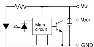
M Photo IC output (Sync light modulation system)
