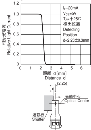
検出位置特性 (2) (参考) Detecting Position Characteristics (2) (Reference)
