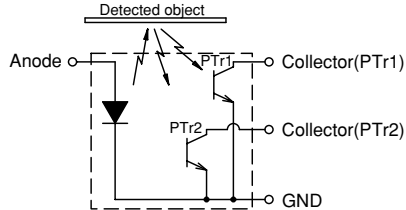
S Regressive Reflection Type Photosensor
