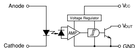
D Photo IC output (Open collector, Light on—Output transistor off)
