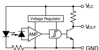
K Photo IC output (With pull-up resistor, Light on—Output transistor off)
