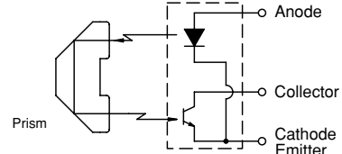
T Regressive Reflection Type Photosensor (cathode and emitter in common)
