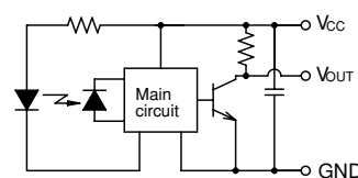
N Photo IC output (Sync light modulation system)
