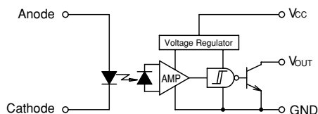
C Photo IC output (Open collector, Light on—Output transistor on)
