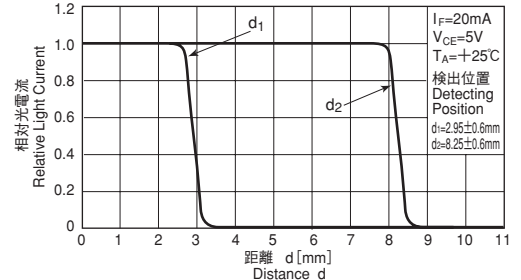
検出位置特性 (2) (参考) Detecting Position Characteristics (2) (Reference)
