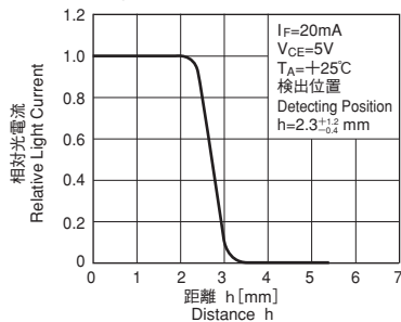
検出位置特性 (1) (参考) Detecting Position Characteristics (1) (Reference)
