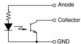
R Phototransistor Output (with limiting resistor)
