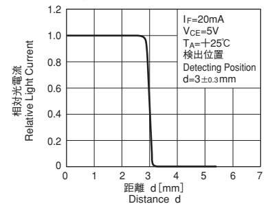
検出位置特性 (2) (参考) Detecting Position Characteristics (2) (Reference)
