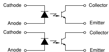
B 2-Gang photointerrupter
