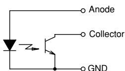
I Photo IC output (Open collector, Light on—Output transistor on)
