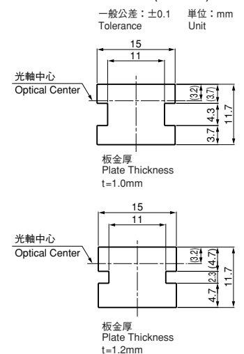
Installation Hole Dimensions (Reference)
